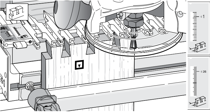
8-40 TD tail boards are clamped vertically in the jig. The inside face of the TD tails is away from the jig body. The finger assembly is in the TD TAILS mode, set on the single \leq 1" [ \leq 26\text{mm} ] setting. There is only one setting in this mode.
